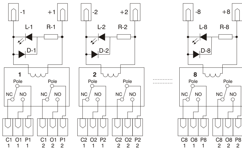
Schematic of TT-IMRB-080230A2S
