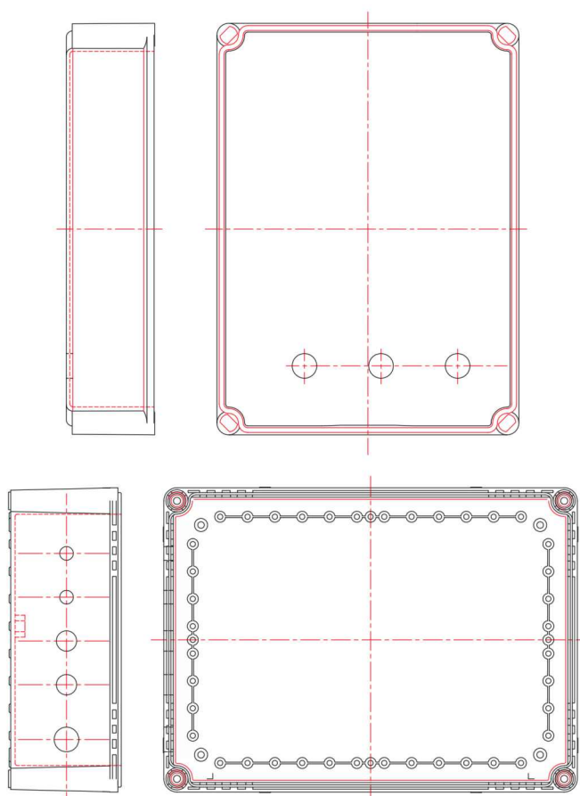
Tailor drilled cable gland holes (Article No. 01 17 00289)
