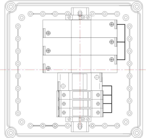
Junction Box (Article No. 01 17 00031)
