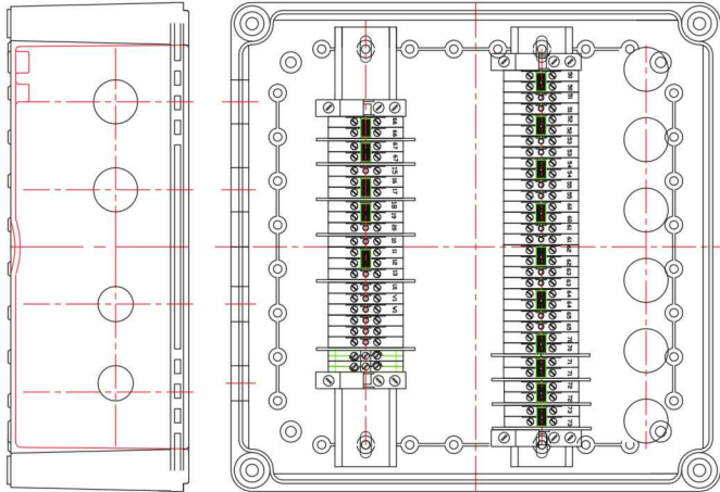
Junction Box (Article No. 01 17 00069)
