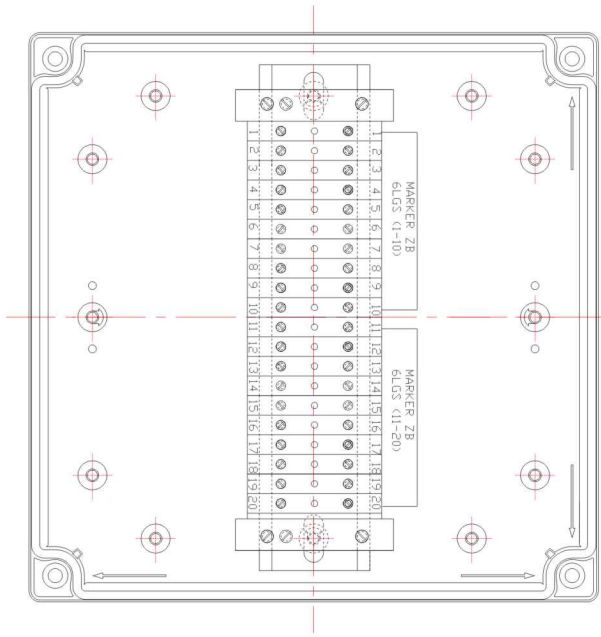
Junction Box (Article No. 01 17 00005)
