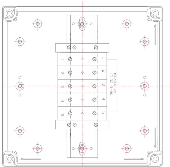
Junction Box (Article No. 01 17 00020)
