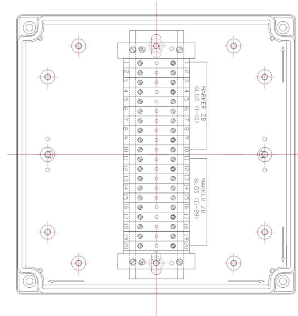
Junction Box (Article No. 01 17 00012)
