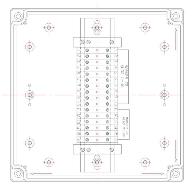
Junction Box (Article No. 01 17 00004)
