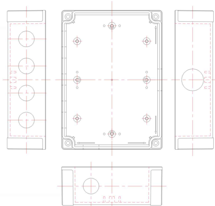
Tailor drilled cable gland holes (Article No. 01 17 00250)
