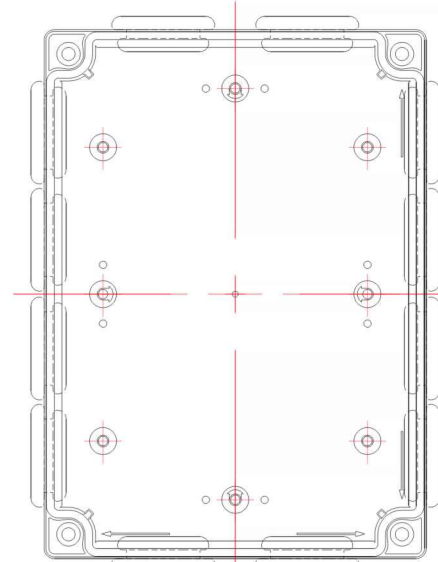
Tailor drilled cable gland holes (Article No. 01 17 00153)
