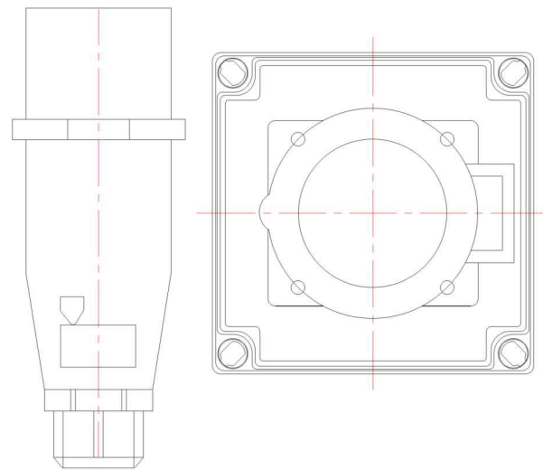
Plug & Socket Unit (Article No. 01 17 00086)
