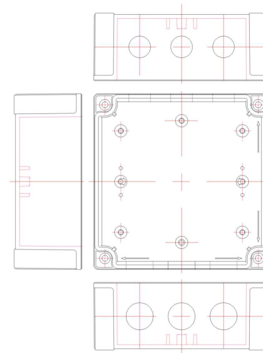
Tailor drilled cable gland holes (Article No. 01 05 00915)
