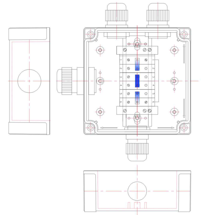
Junction Box (Article No. 01 17 00072)
